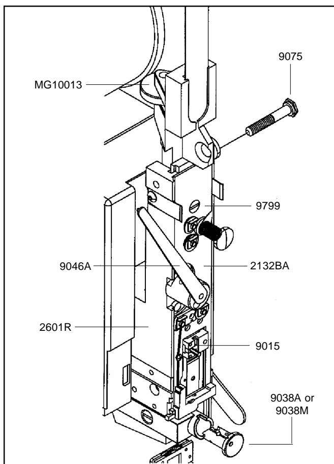
Figure 6 - Adjusting the Left Leg and Wire Draw
